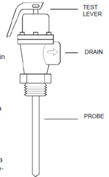
Typical T&P Valve
